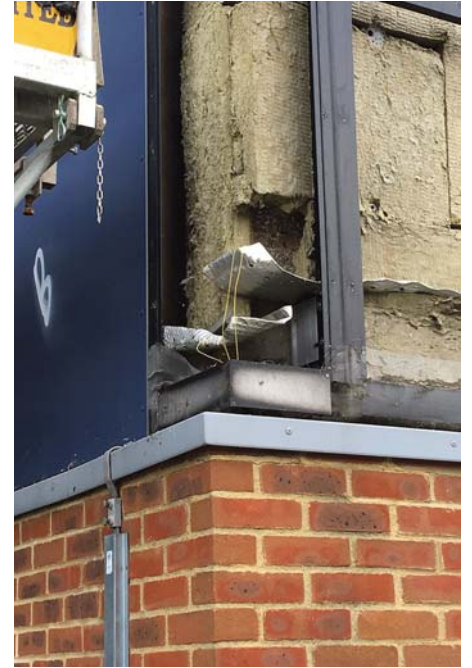
Incorrectly installed firebreaks and gaps in insulation.
